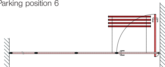
Parking position 6
