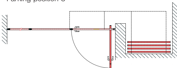
Parking position 3
