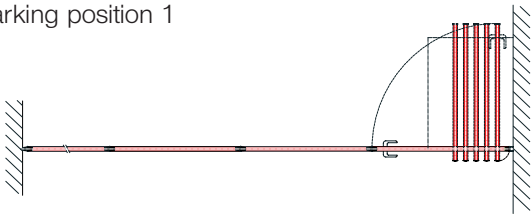
Parking position 1
